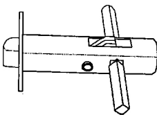
(e) Latch with spindle installed on "the diamond"
