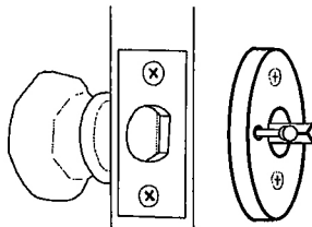
(f) Spindle with 1 doorknob
