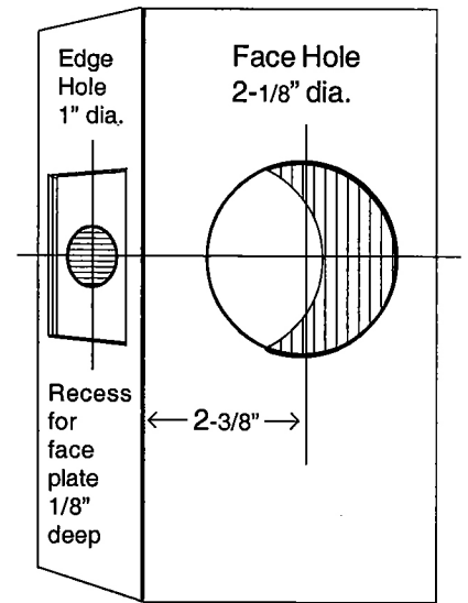
(a) Standard sizes of pre-drilled holes
