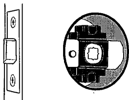
(b) Latch w/ face-plate + alignment pc
