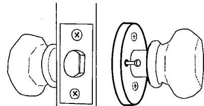
(g) Fully assembled latch set
